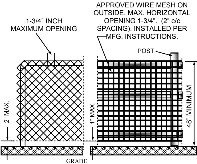
FIGURE 3 CHAIN LINK
