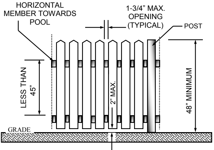
FIGURE 2- PICKET FENCE
