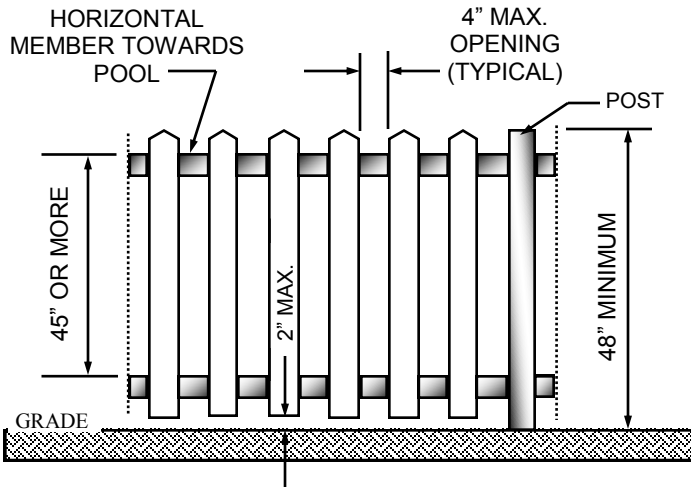
FIGURE 1- PICKET FENCE
